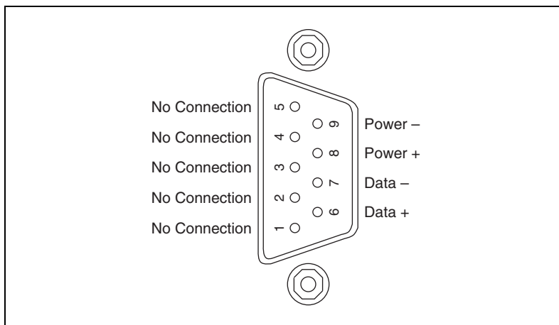
Figure 3-3. Fieldbus Connector Pinout
