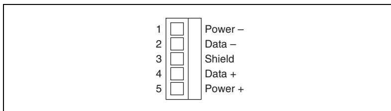
Figure 3-4. Screw Terminal Block Pinout
