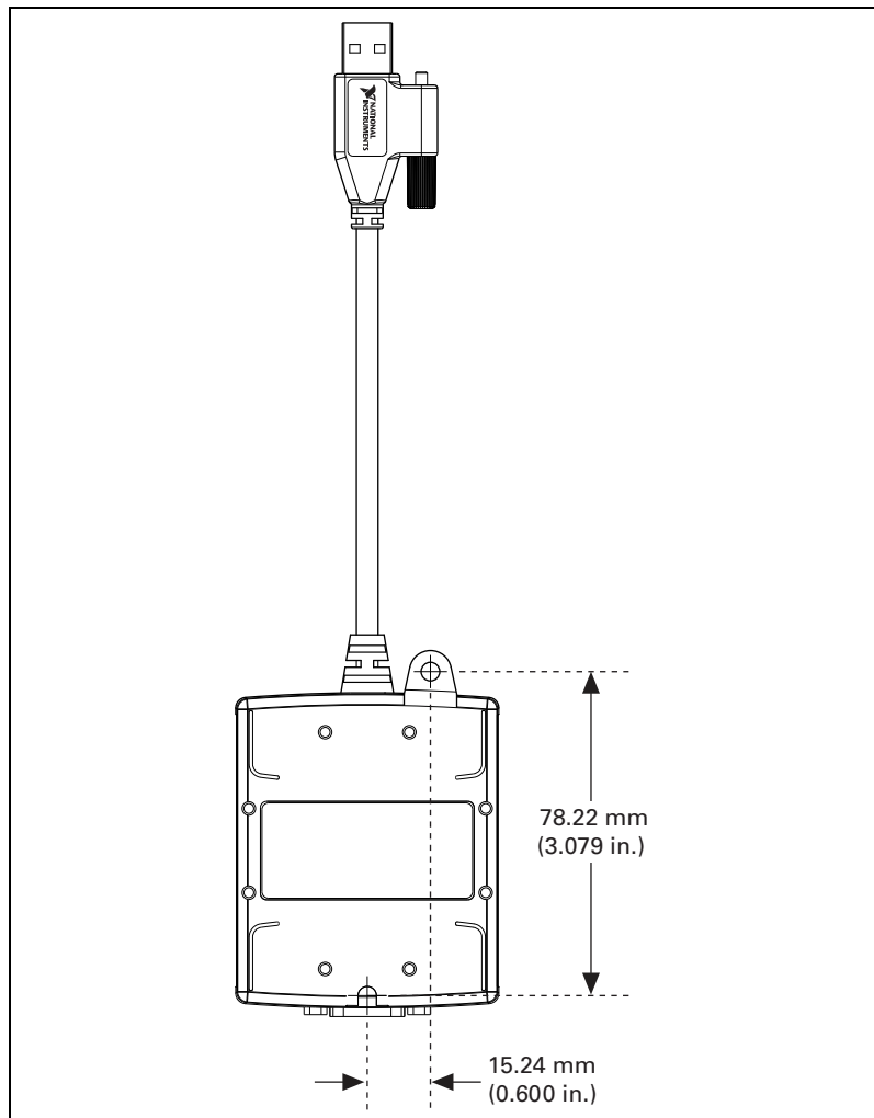
Figure 2-8. Dimensions of the Mounting Tab and Notch
